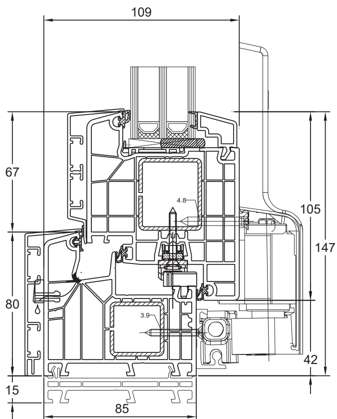
Blendrahmen 180x05/ S12639 Flügel Classic 180x30/ S12638
