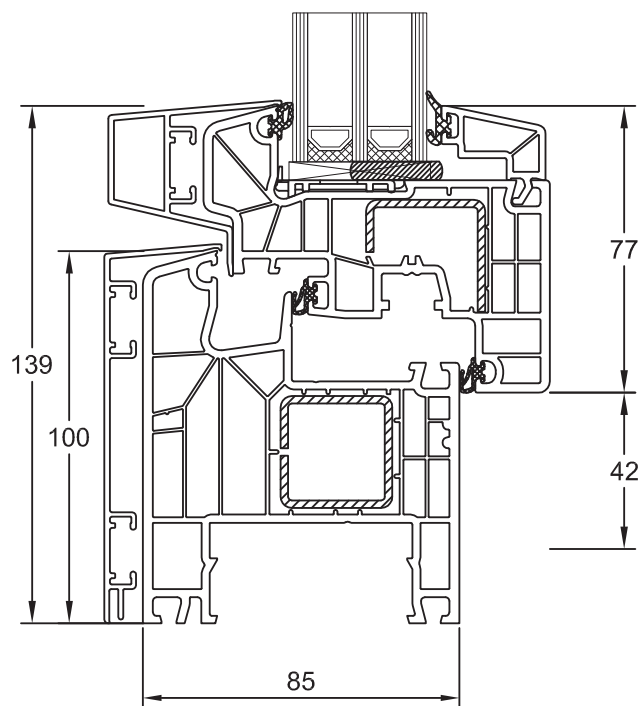
Blendrahmen 180x04/ S12630 Flügel hfv+ 8mm 180x26/ S12639
