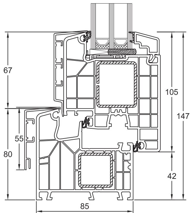
Blendrahmen 180x05/ S12692 Flügel Classic 180x20/ S12631
