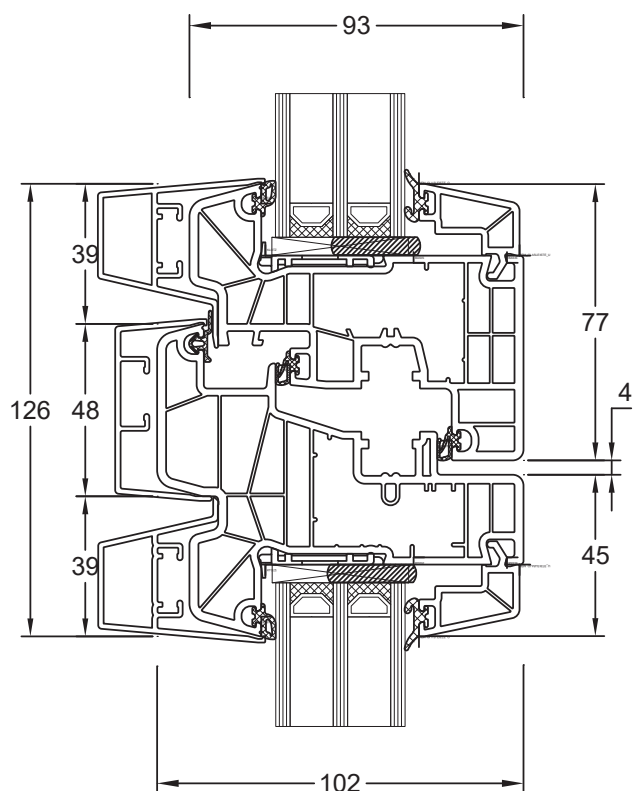
Stulpflügel 180x+69/ S12633+ S12648 Flügel hfv+ 8mm 180x26/ S12639
