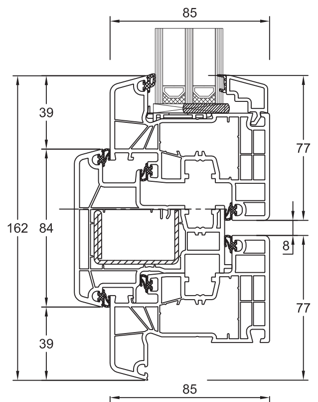
Stulp 180x66 Flügel Classic 180x20
