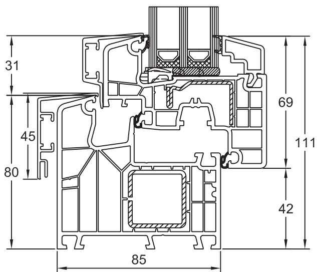
Blendrahmen 180x05/ S12628 Flügel Classic 180x24/ S12649
