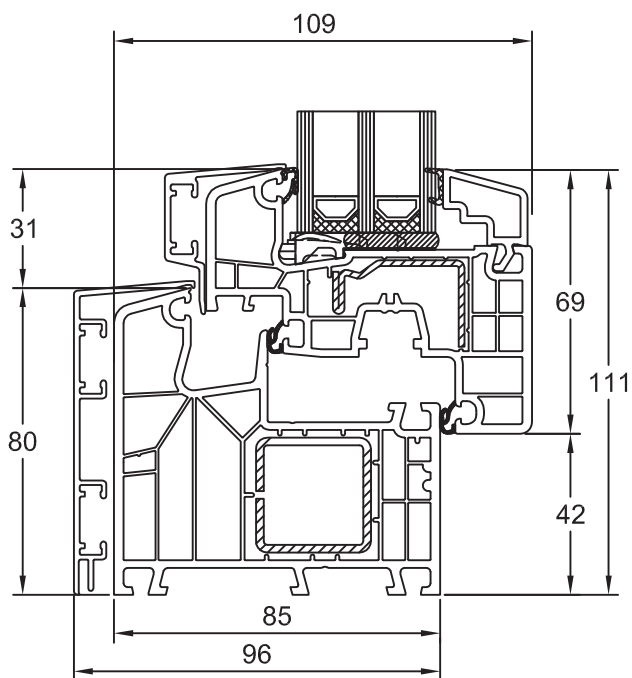
Blendrahmen 180x05/ S12629 Flügel Classic 180x24/ S12649
