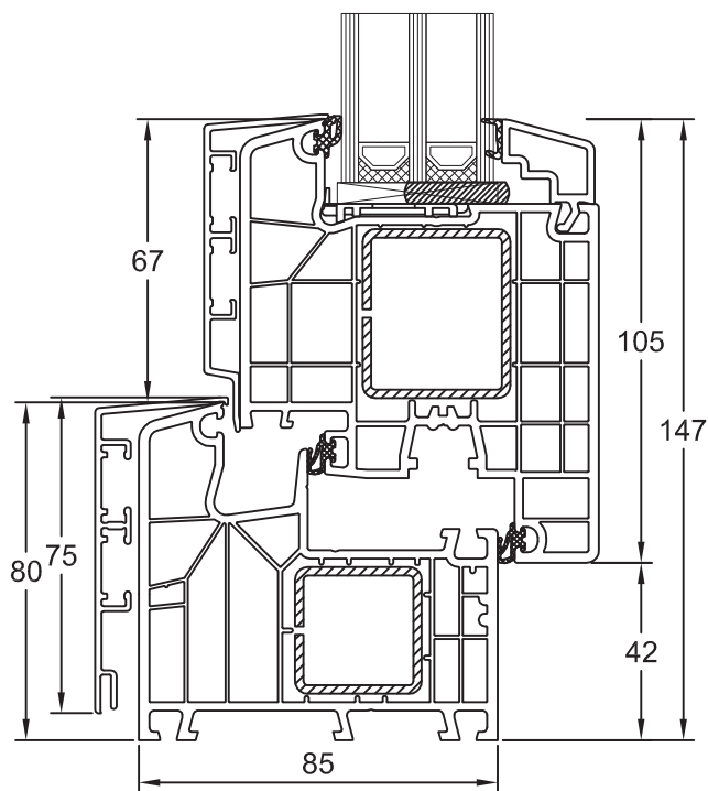
Blendrahmen 180x05/ S12694 Flügel Classic 180x20/ S12631
