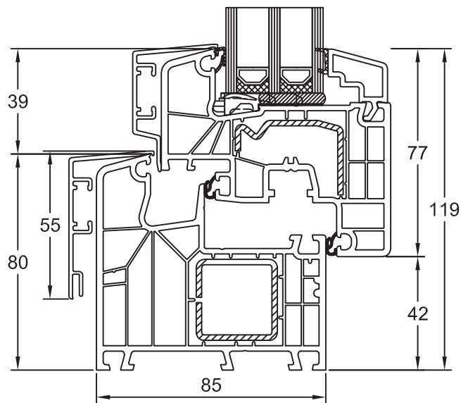
Blendrahmen 180x05/ S12692 Flügel Classic 180x20/ S12631
