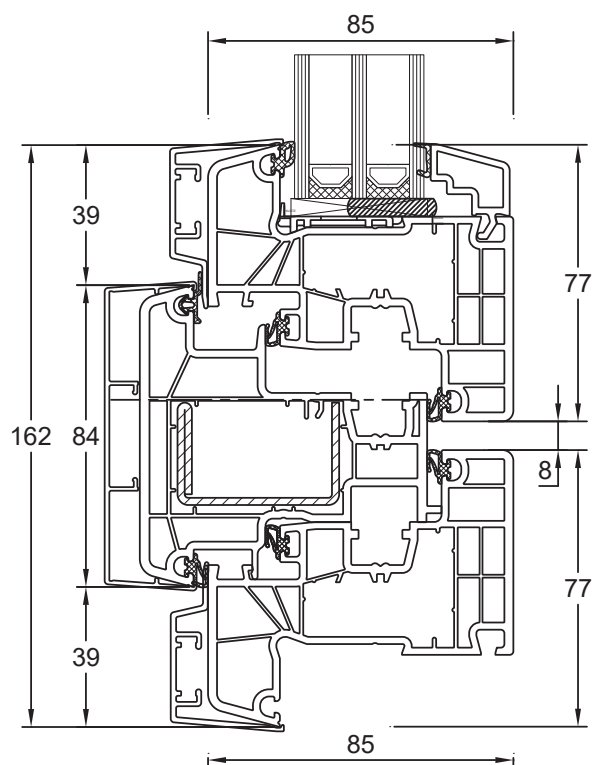
Stulp 180x66/ S12635 Flügel Classic 180x20/ S12631
