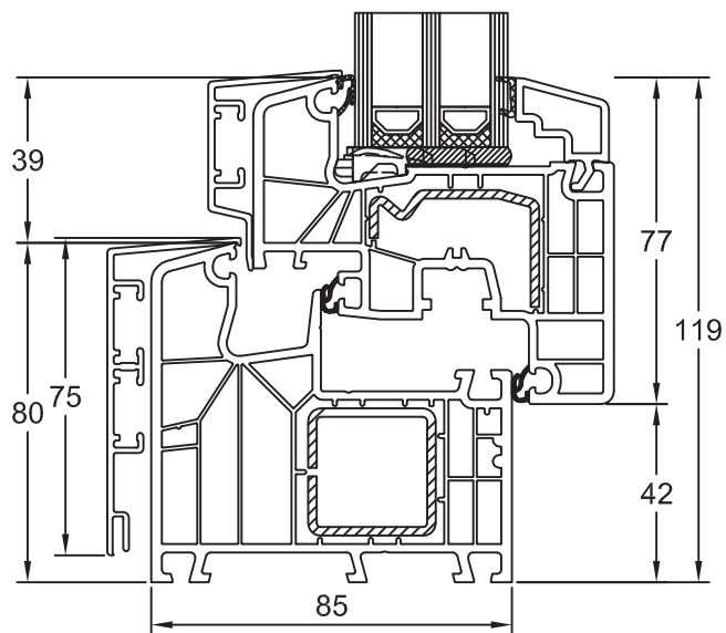
Blendrahmen 180x05/ S12694 Flügel Classic 180x20/ S12631
