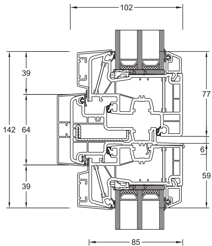
Stulp 180x64 Flügel Classic 080x20
