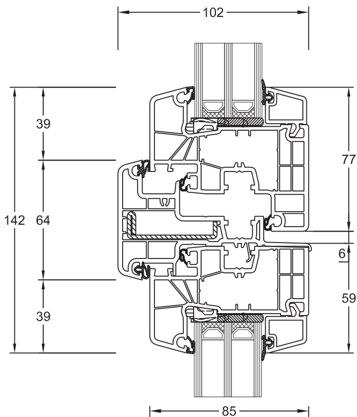
Stulp 180x64 Flügel Classic 180x20
