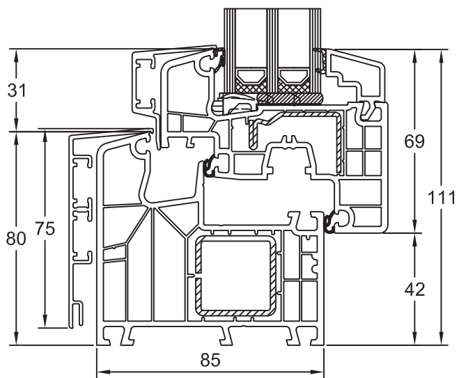
Blendrahmen 180x05/ S12694 Flügel Classic 180x24/ S12629
