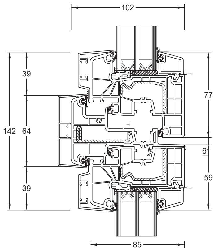
Stulp 180x64/ S12634 Flügel Classic 180x20/ S12631
