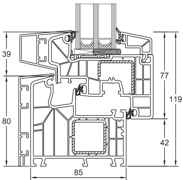
Blendrahmen 180x05/ S12929 Flügel hfv+ 8 mm 180x26/ S12639
